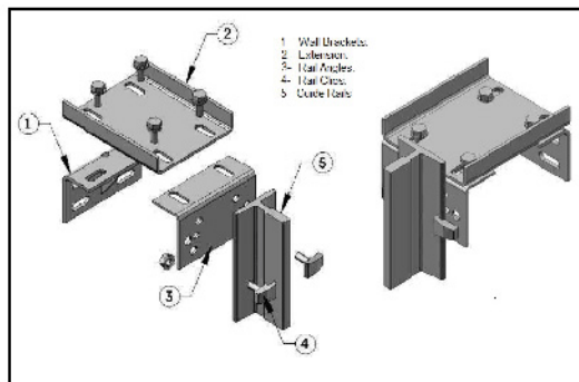
Wall Bracket
