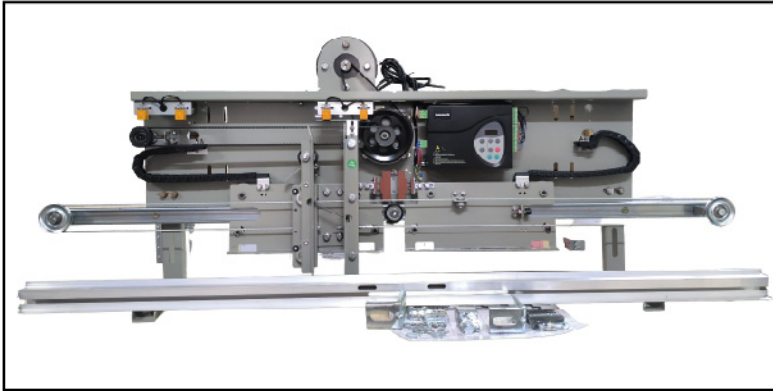
Door Operator
